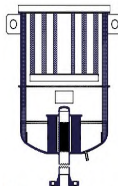
Diffuser and absorption silencer with noise and heat insulation SDAA
