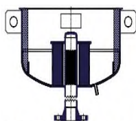
Diffuser silencer with noise and thermal insulation SDA
