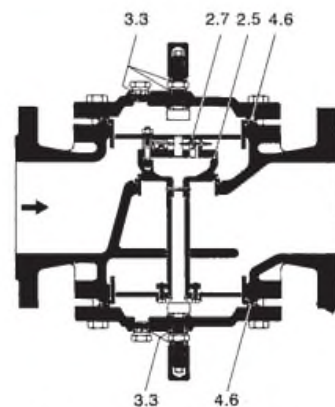
TK 23 and TK 24, DN 65-100 mm (2½-4")
